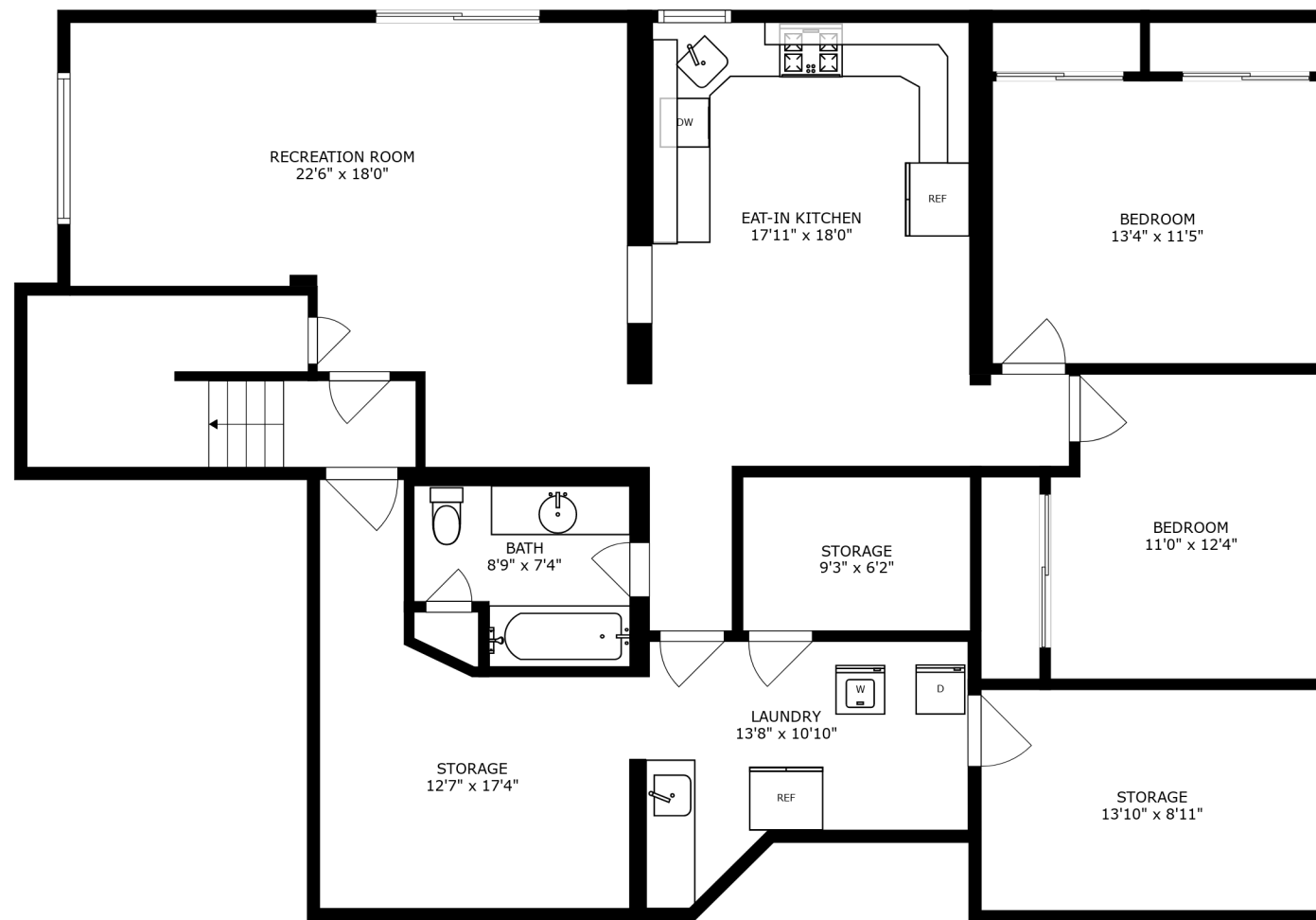
FLOOR 1
