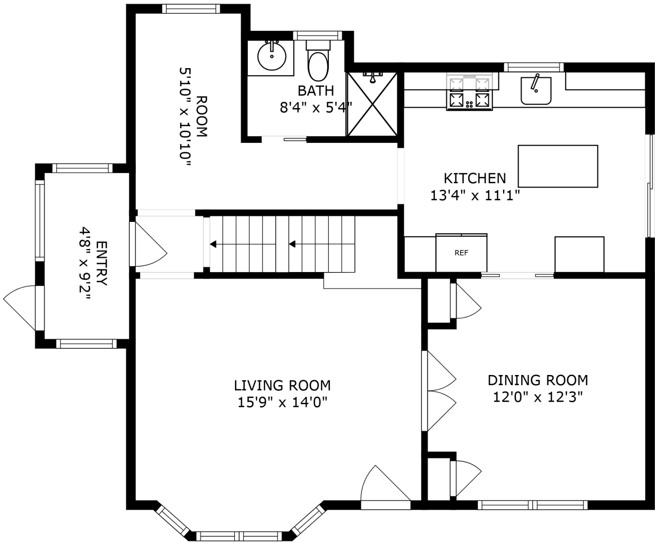
FLOOR 2
