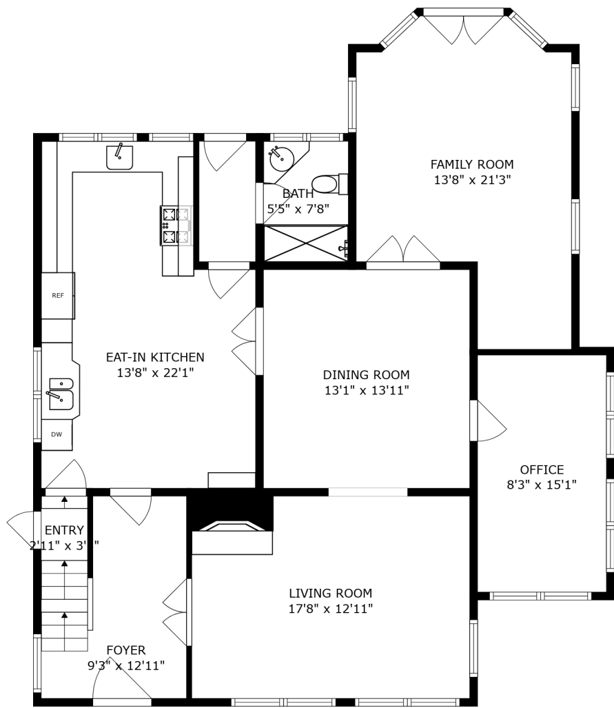
FLOOR 2
