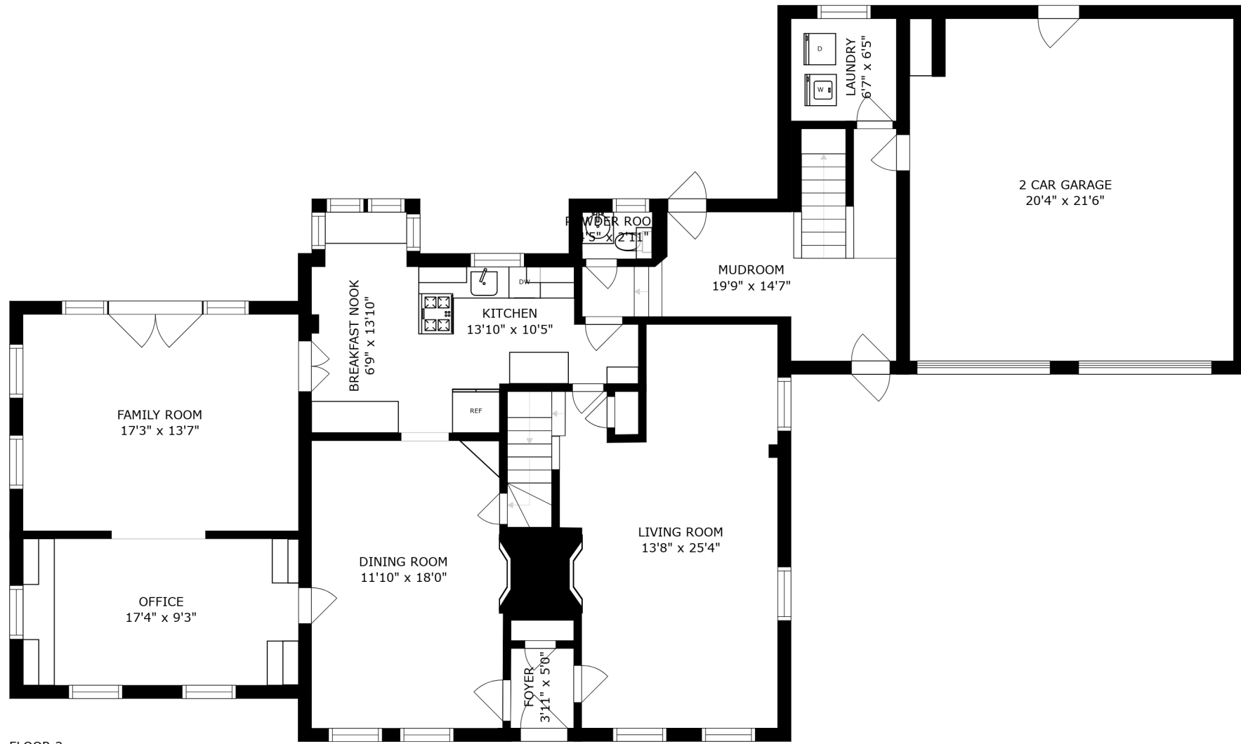
FLOOR 2
