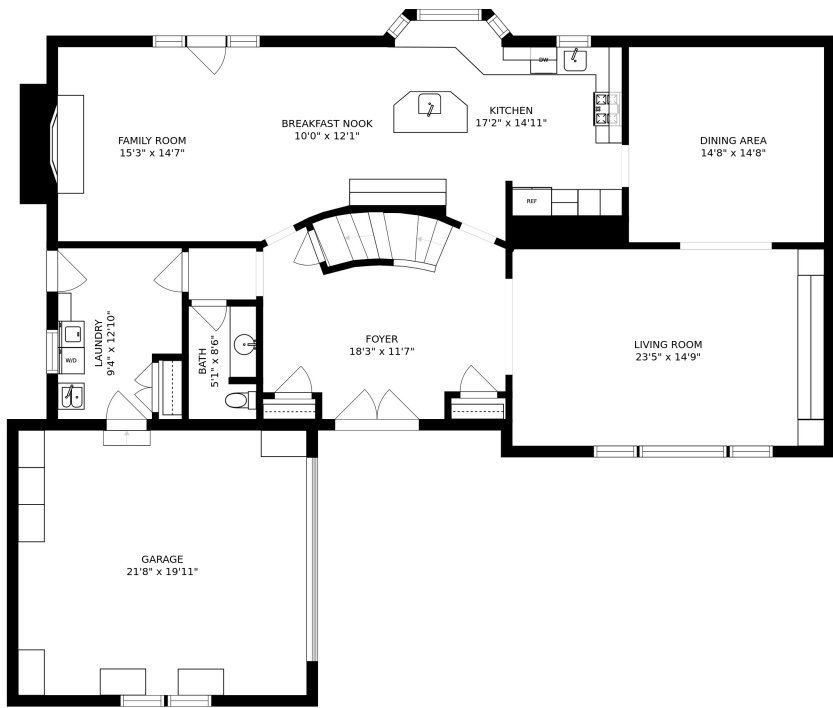
FLOOR 2
