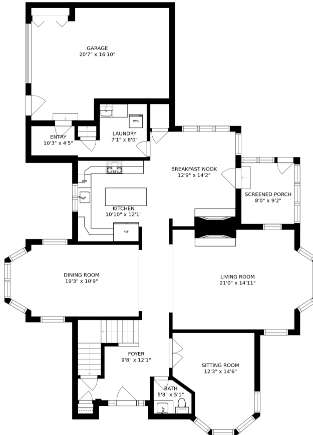
FLOOR 2 = 1362 SQ.FEET
