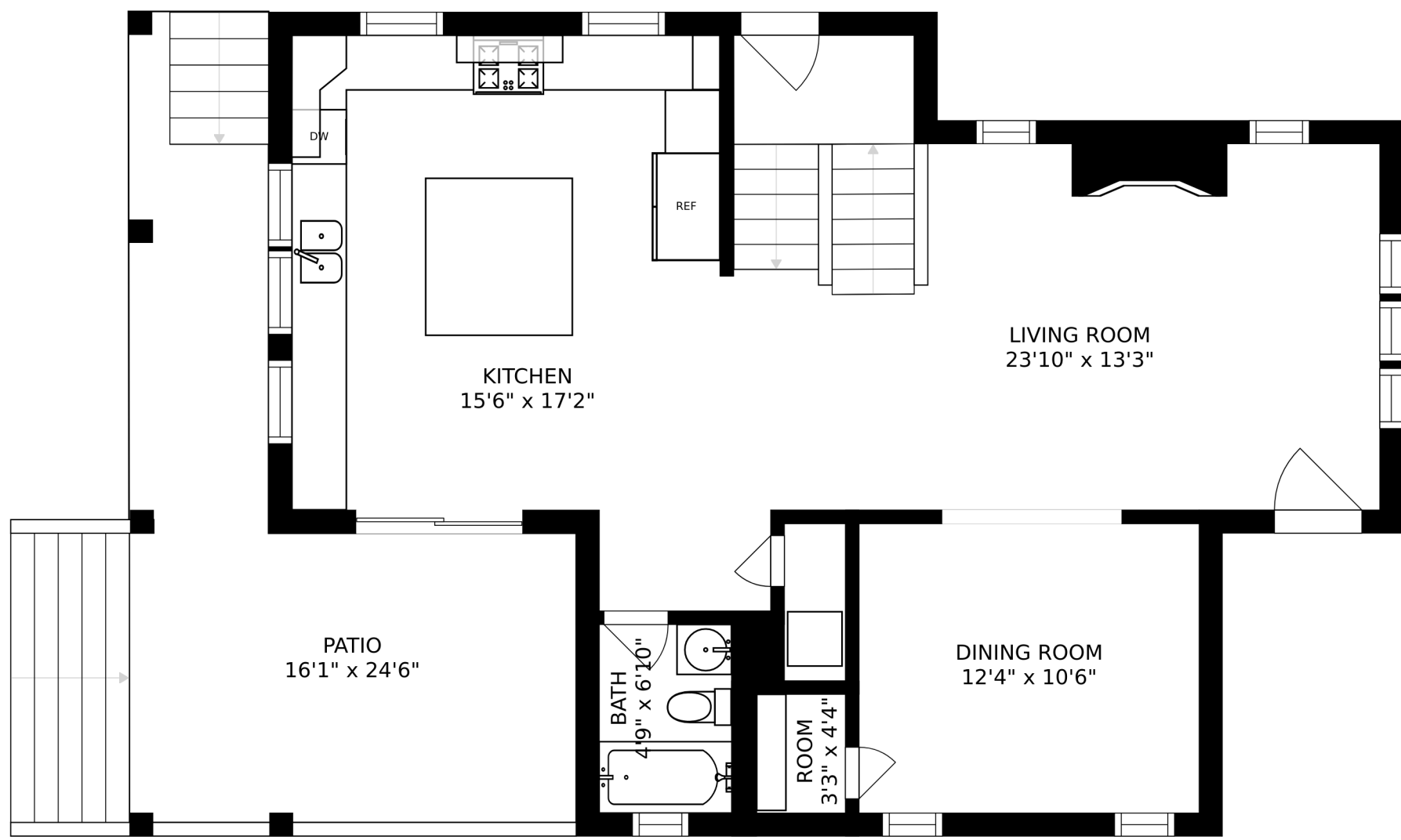
FLOOR 2
