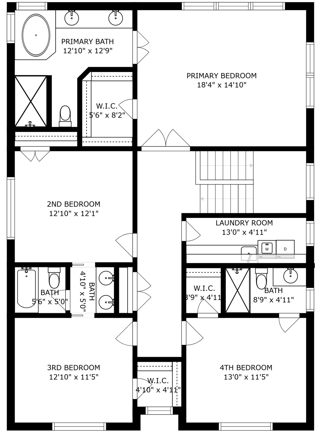
FLOOR 3
