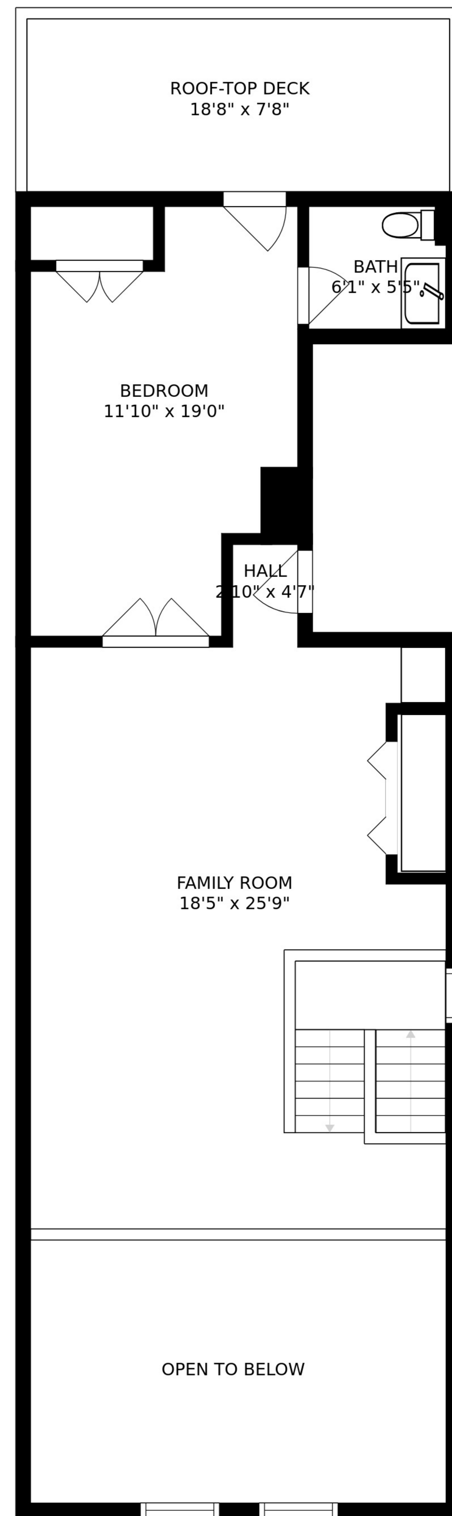
FLOOR 2
