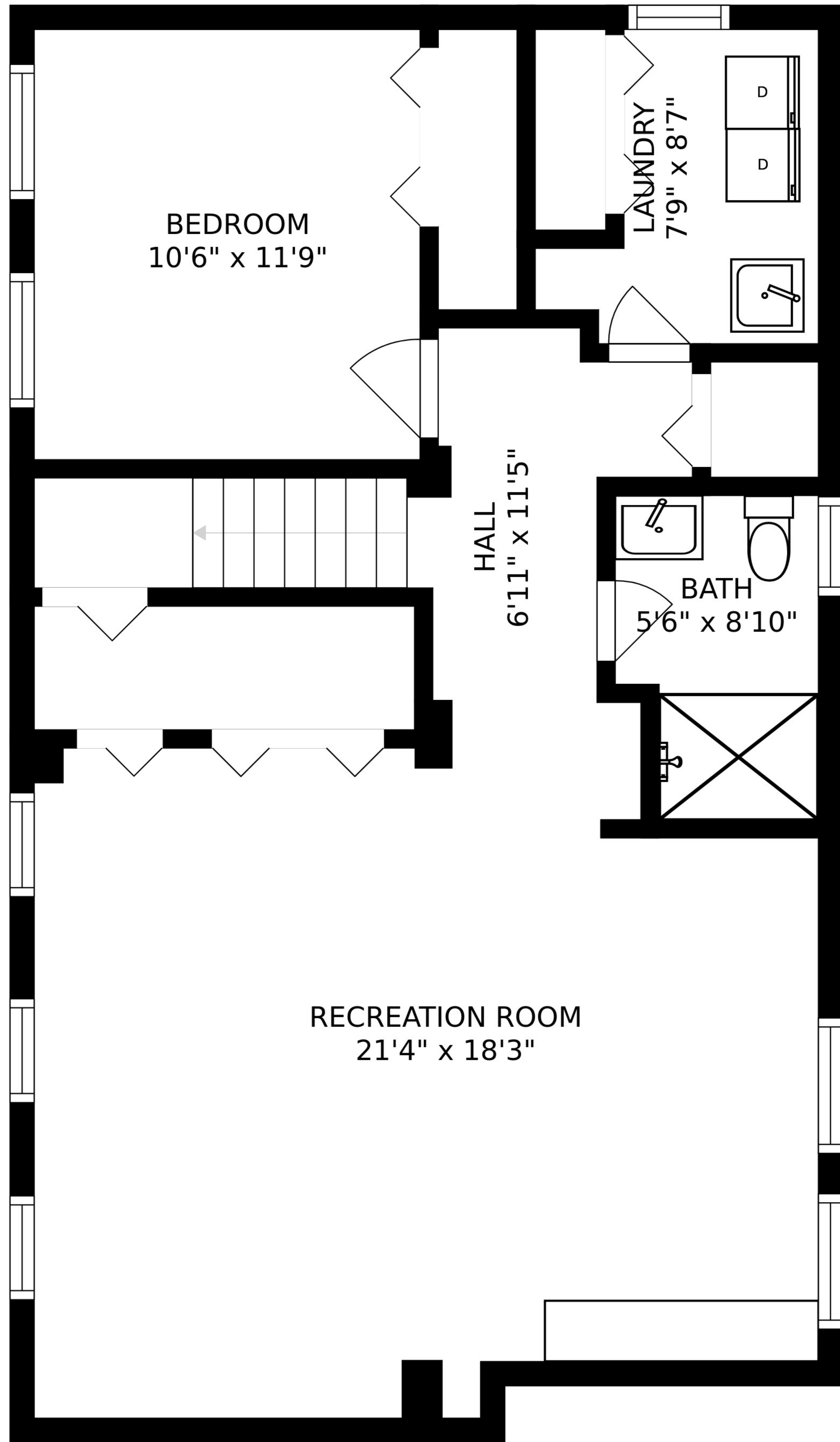
FLOOR 1
