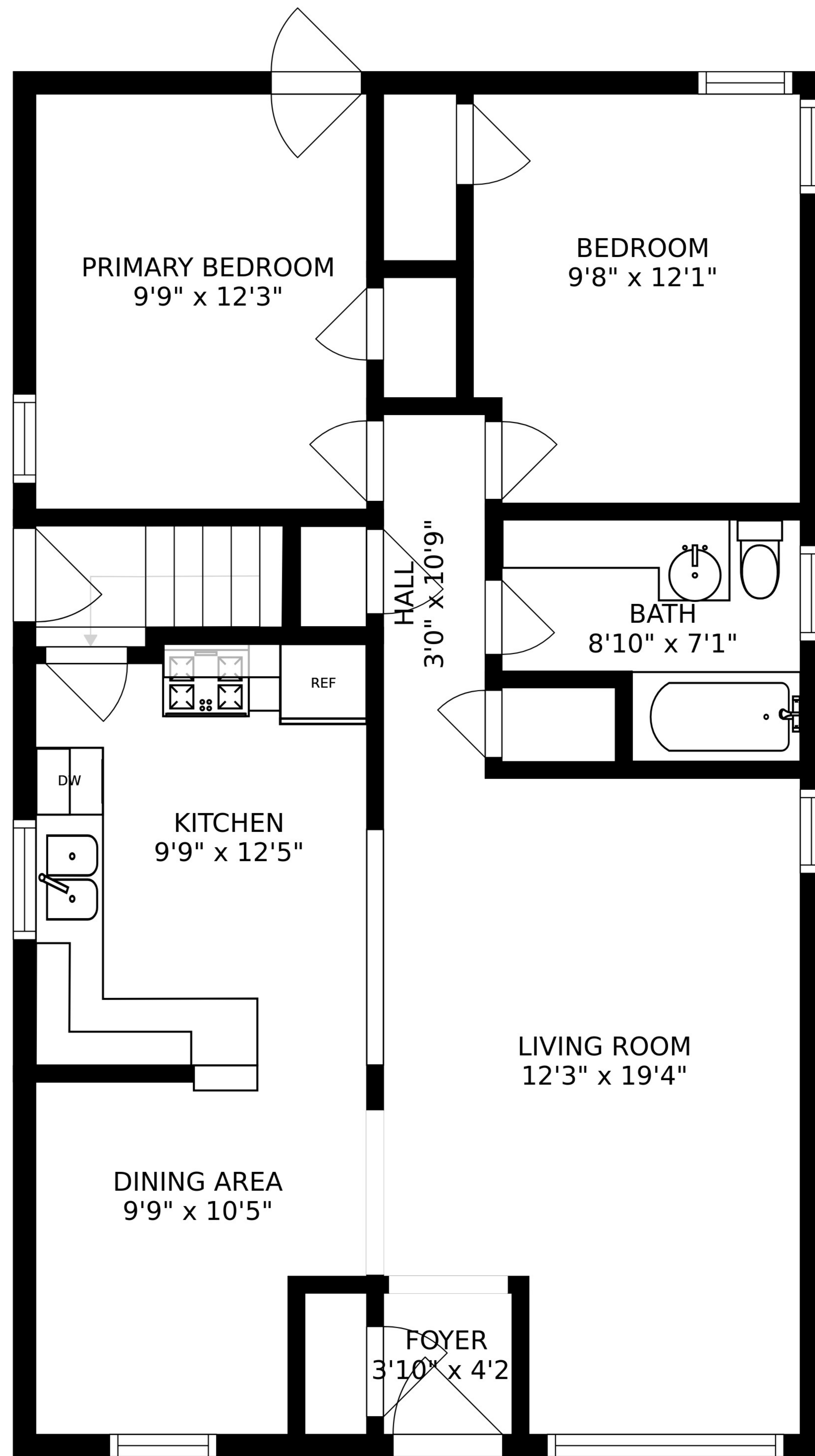
FLOOR 2
