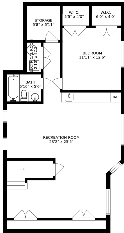
FLOOR 1
