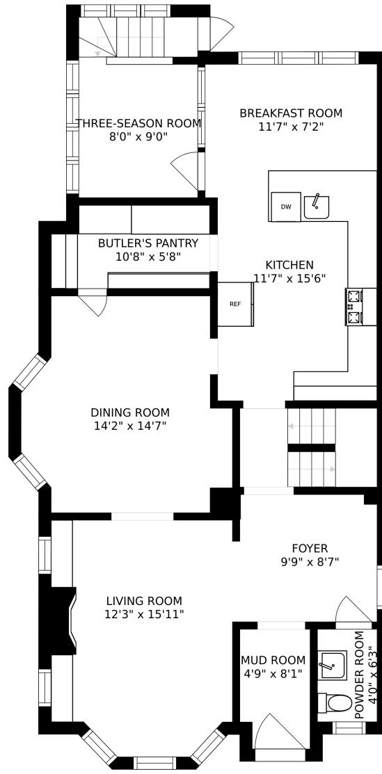
FLOOR 2
