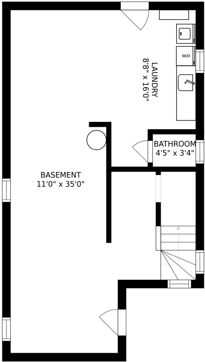
FLOOR 1
