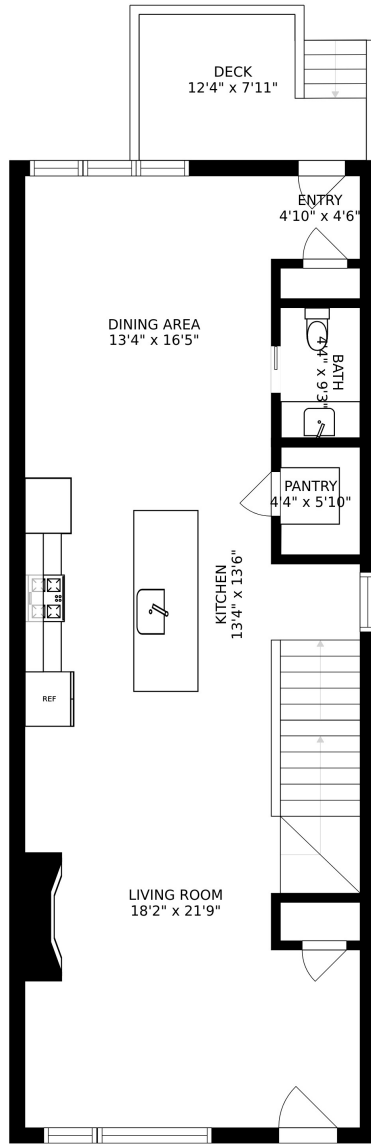
FLOOR 2
