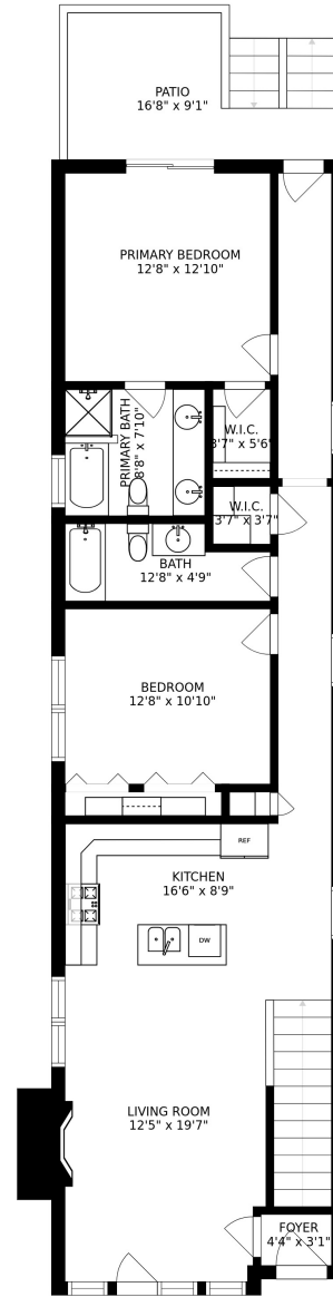
FLOOR 2
