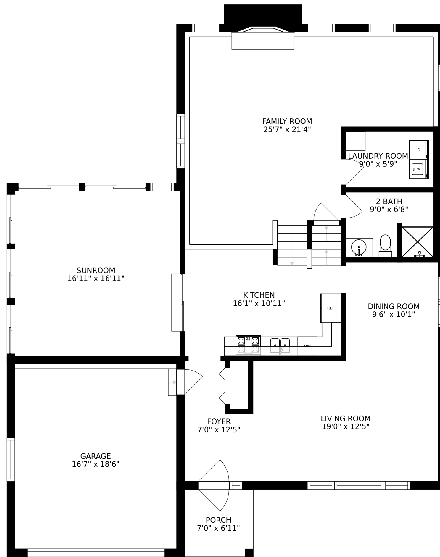
FLOOR 2
