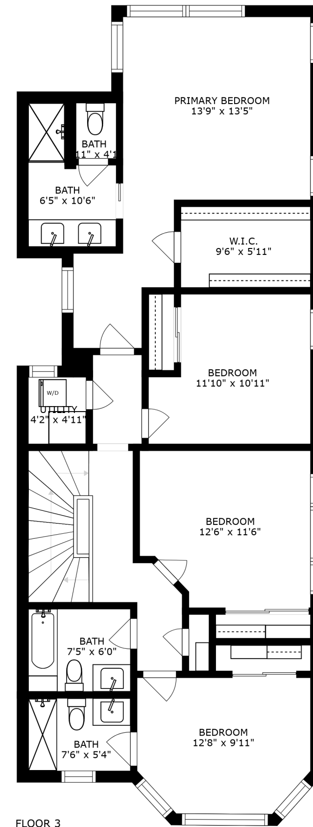
FLOOR 3
