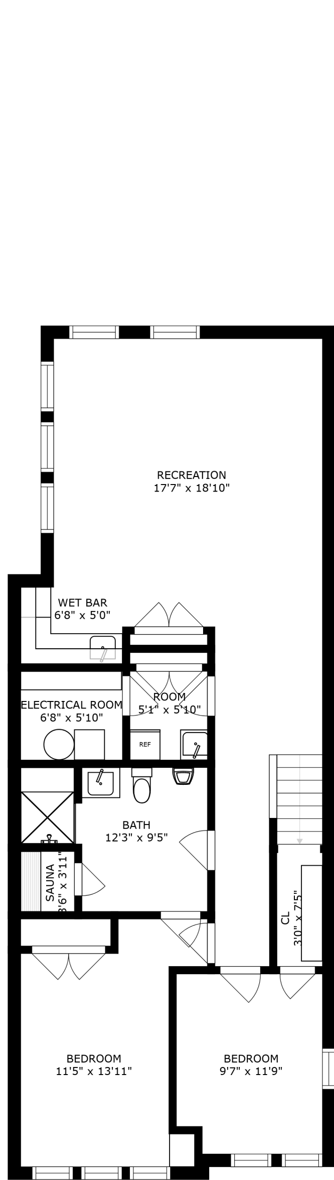
FLOOR 1
