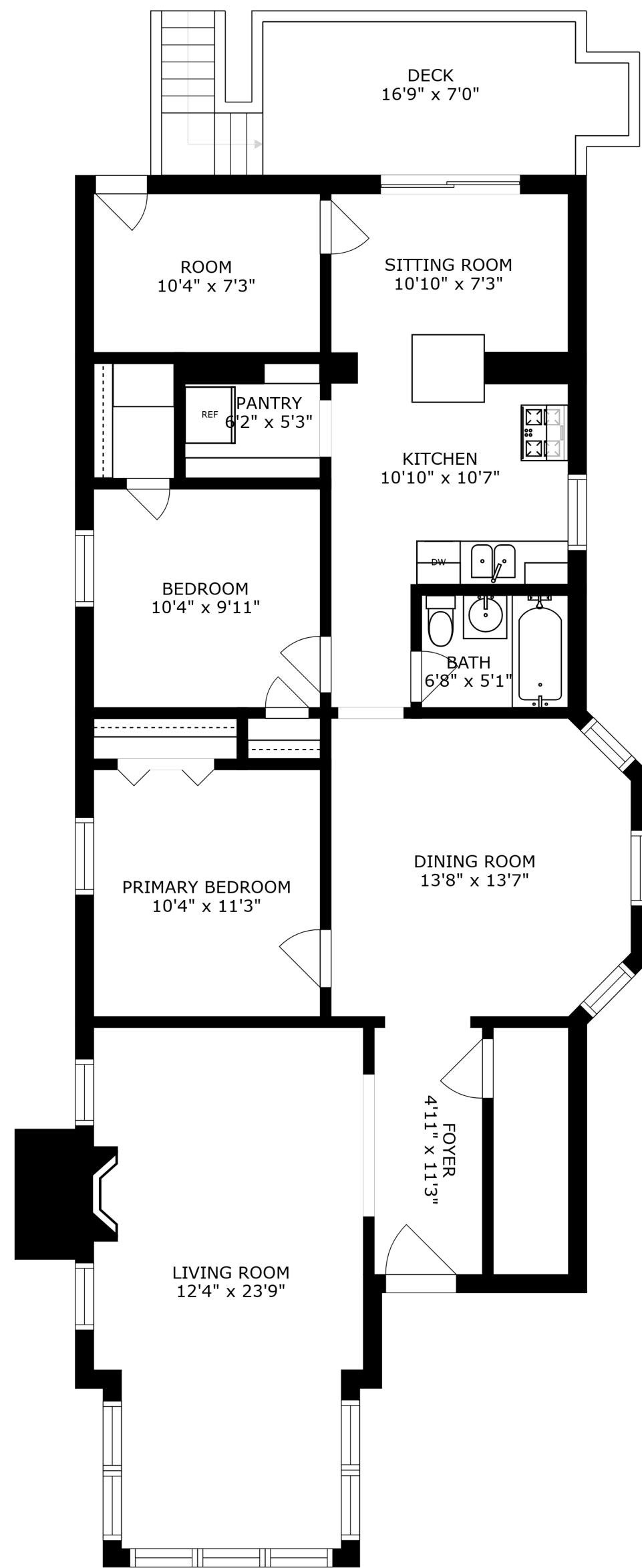
FLOOR 1
