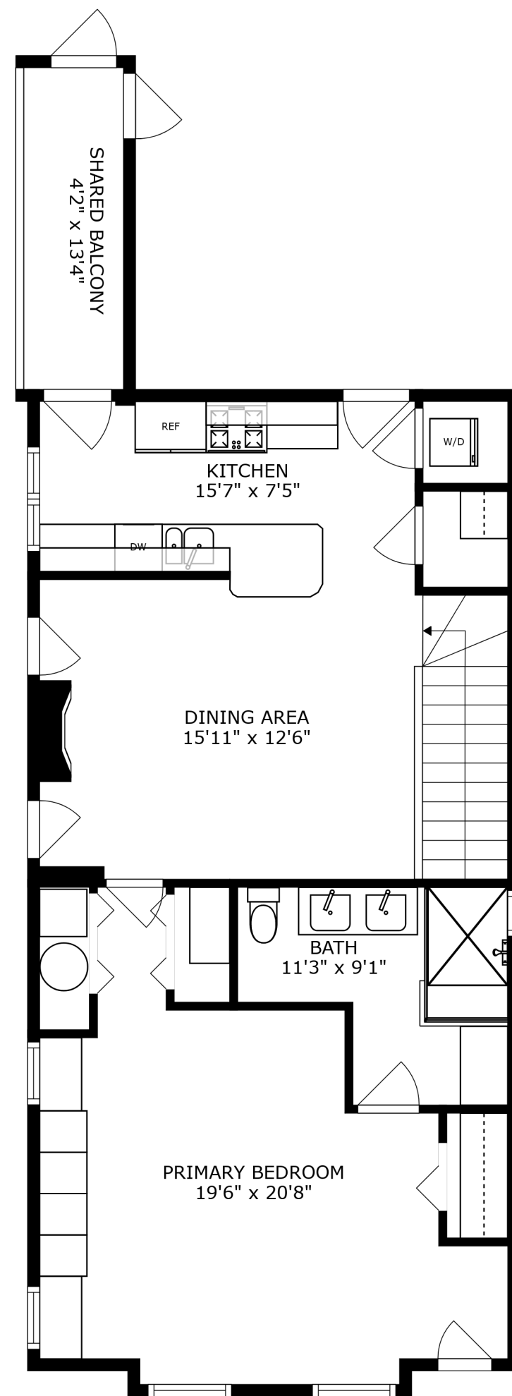
FLOOR 2
