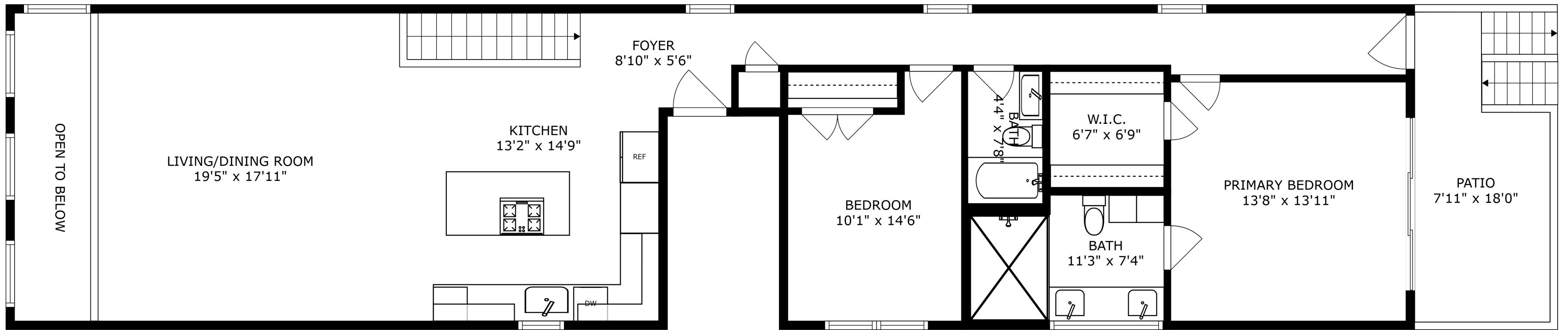
FLOOR 2
