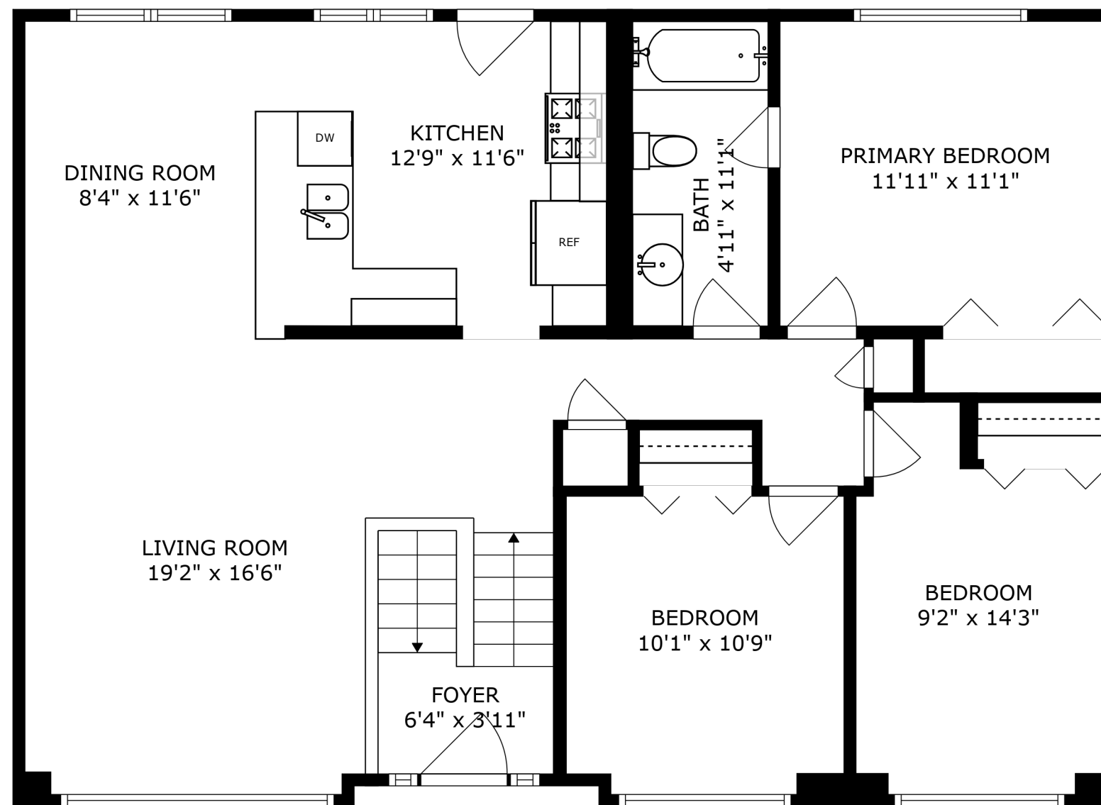
FLOOR 2
