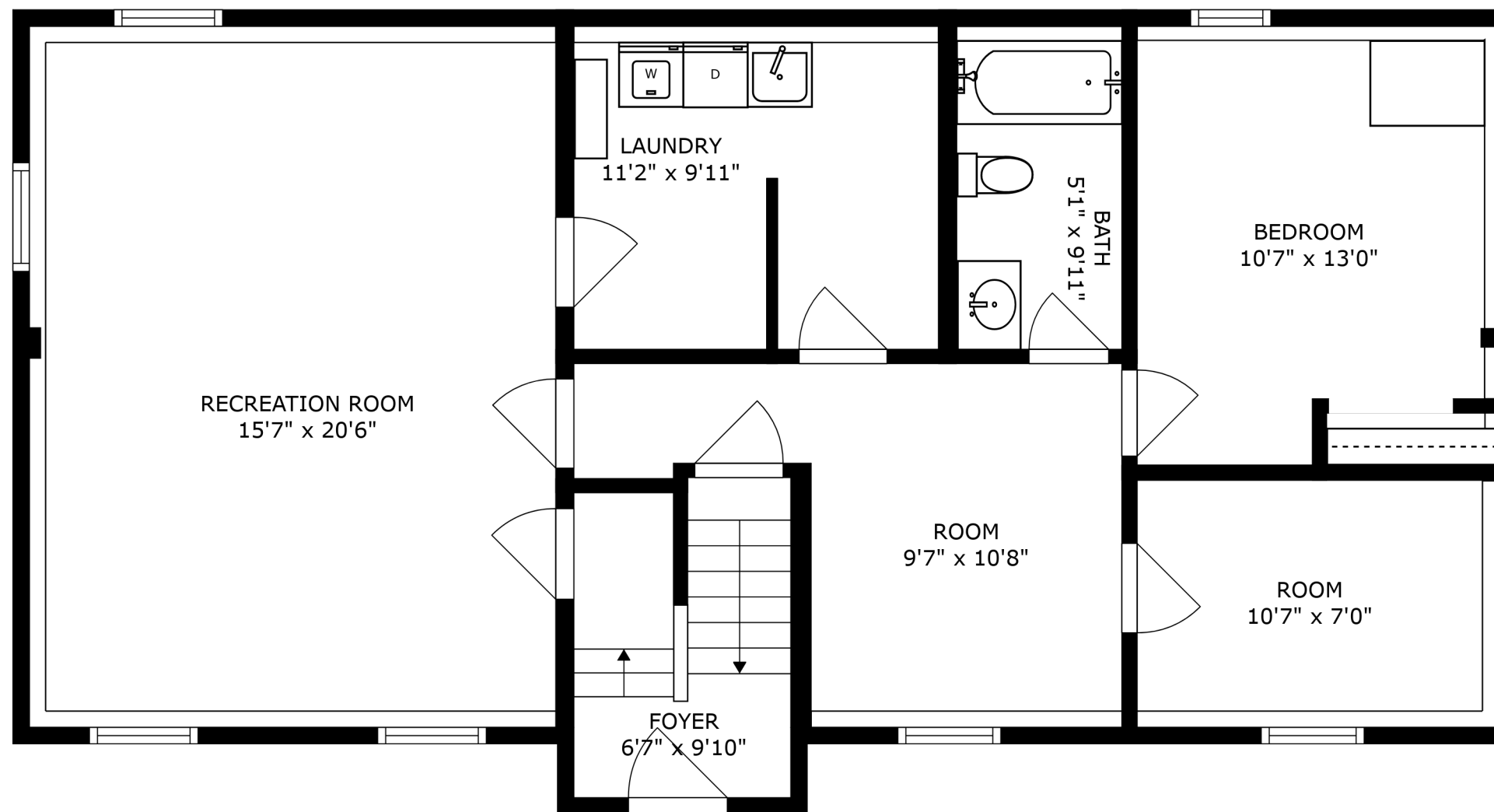
FLOOR 1
