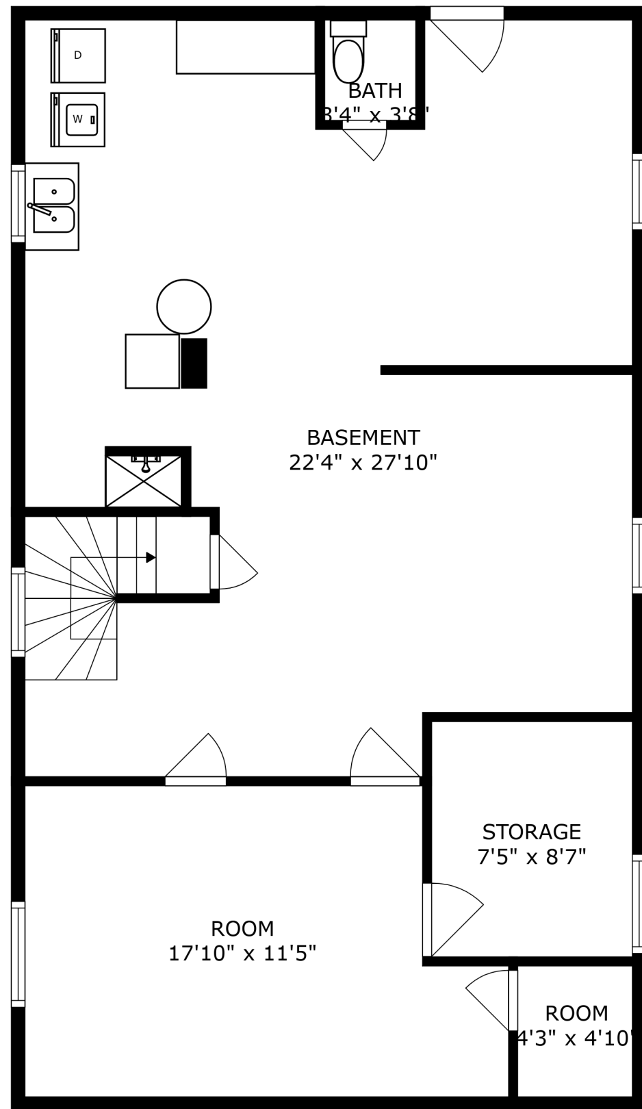
FLOOR 1
