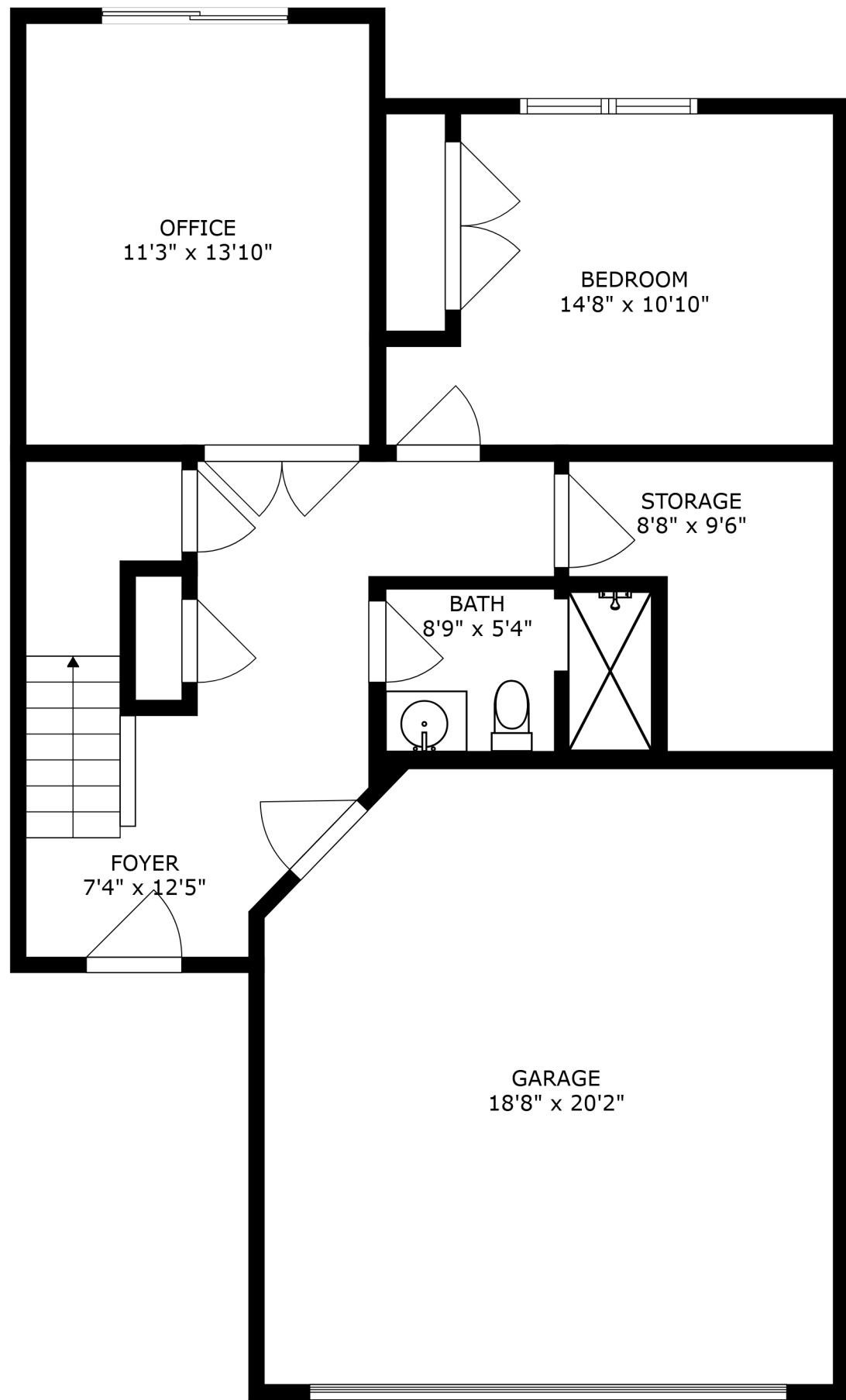
FLOOR 1
