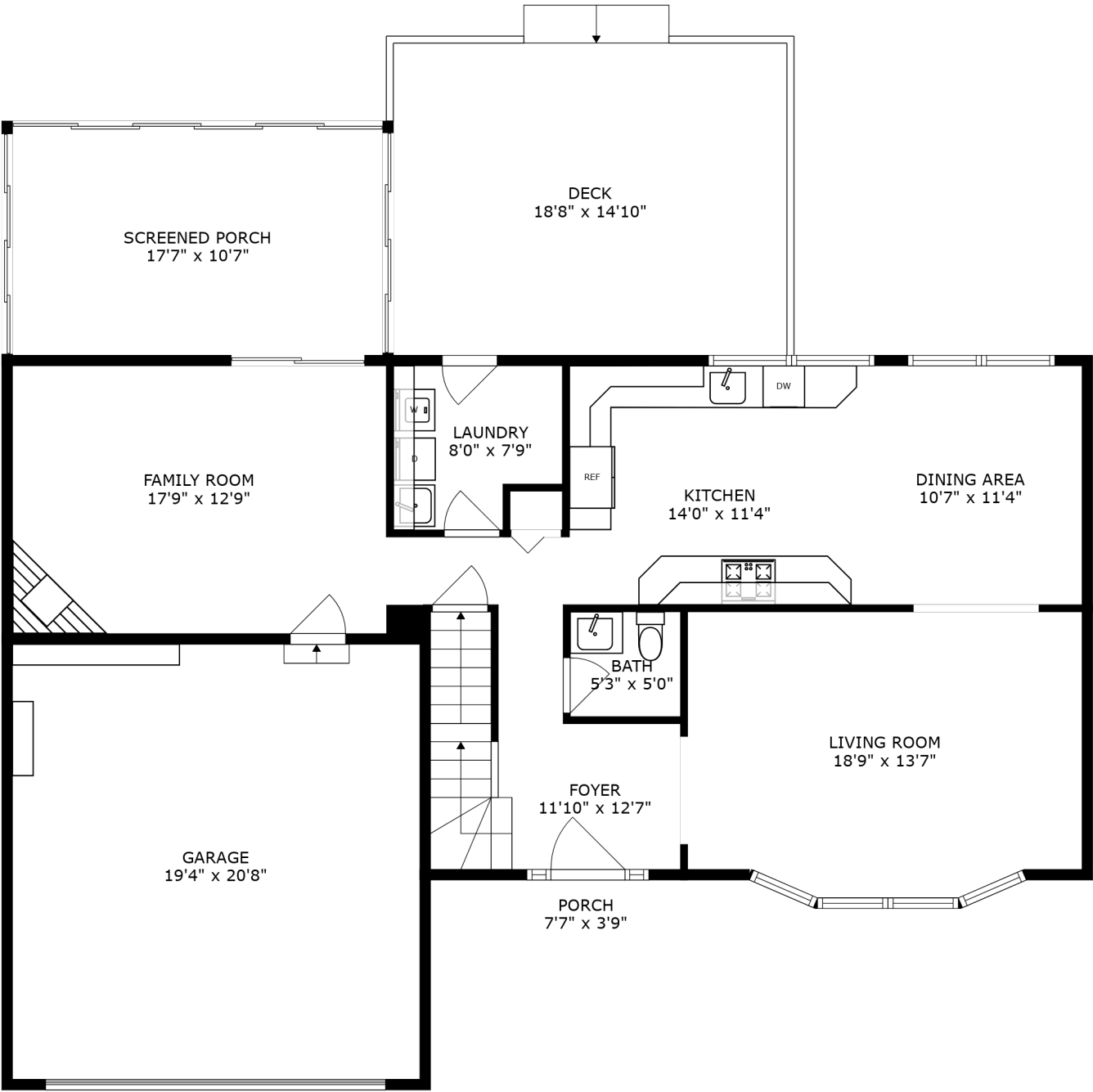
FLOOR 2
