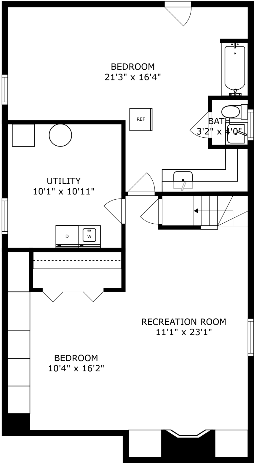
FLOOR 1
