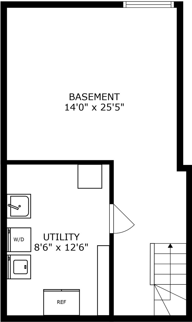
FLOOR 1
