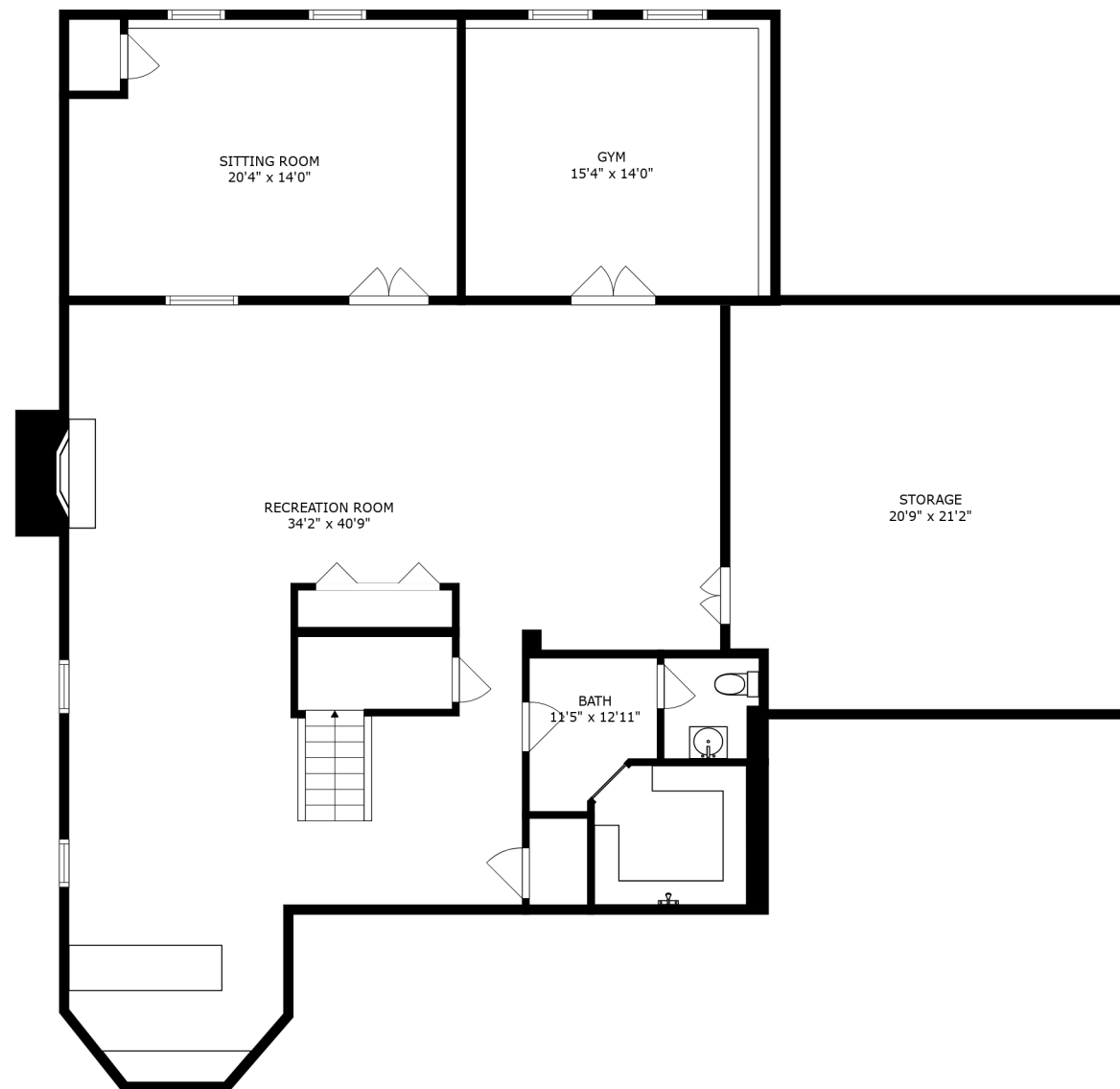
FLOOR 1
