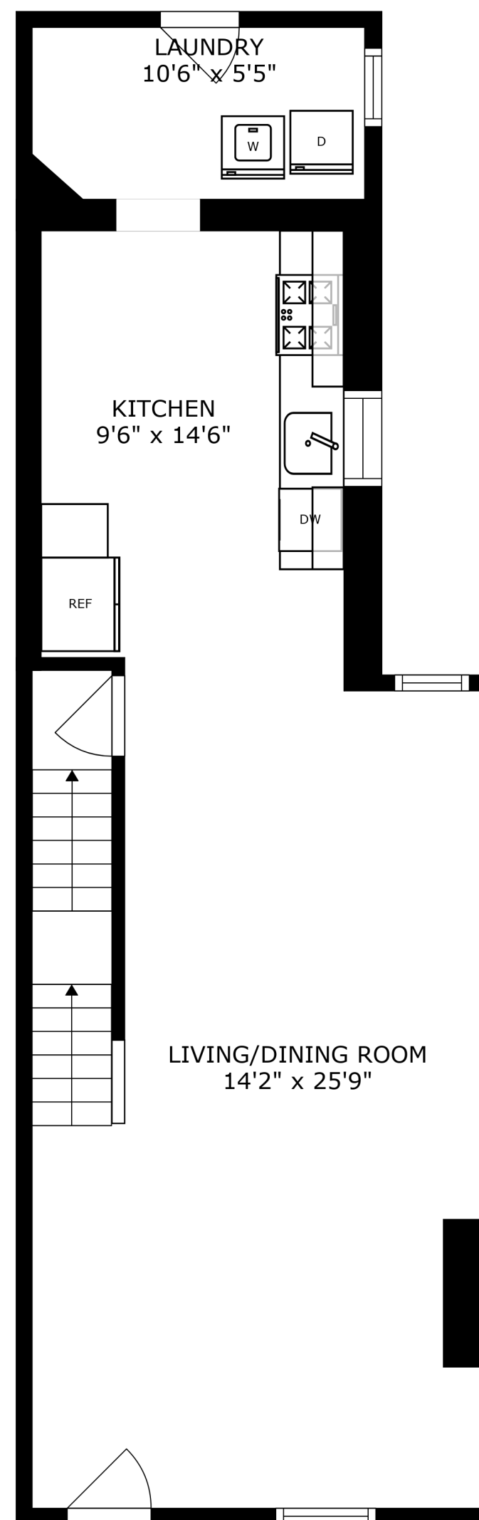
FLOOR 2
