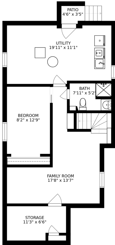
FLOOR 1
