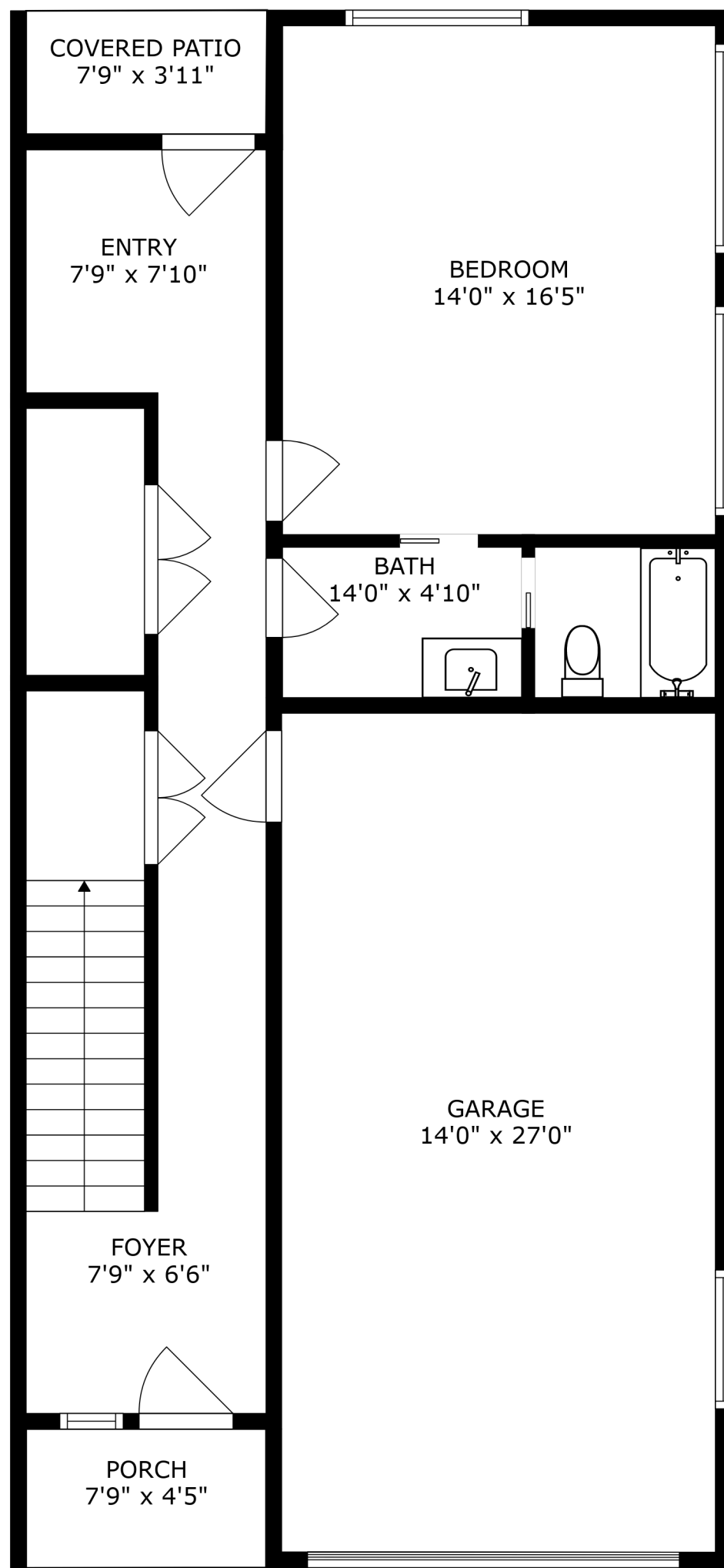
FLOOR 1
