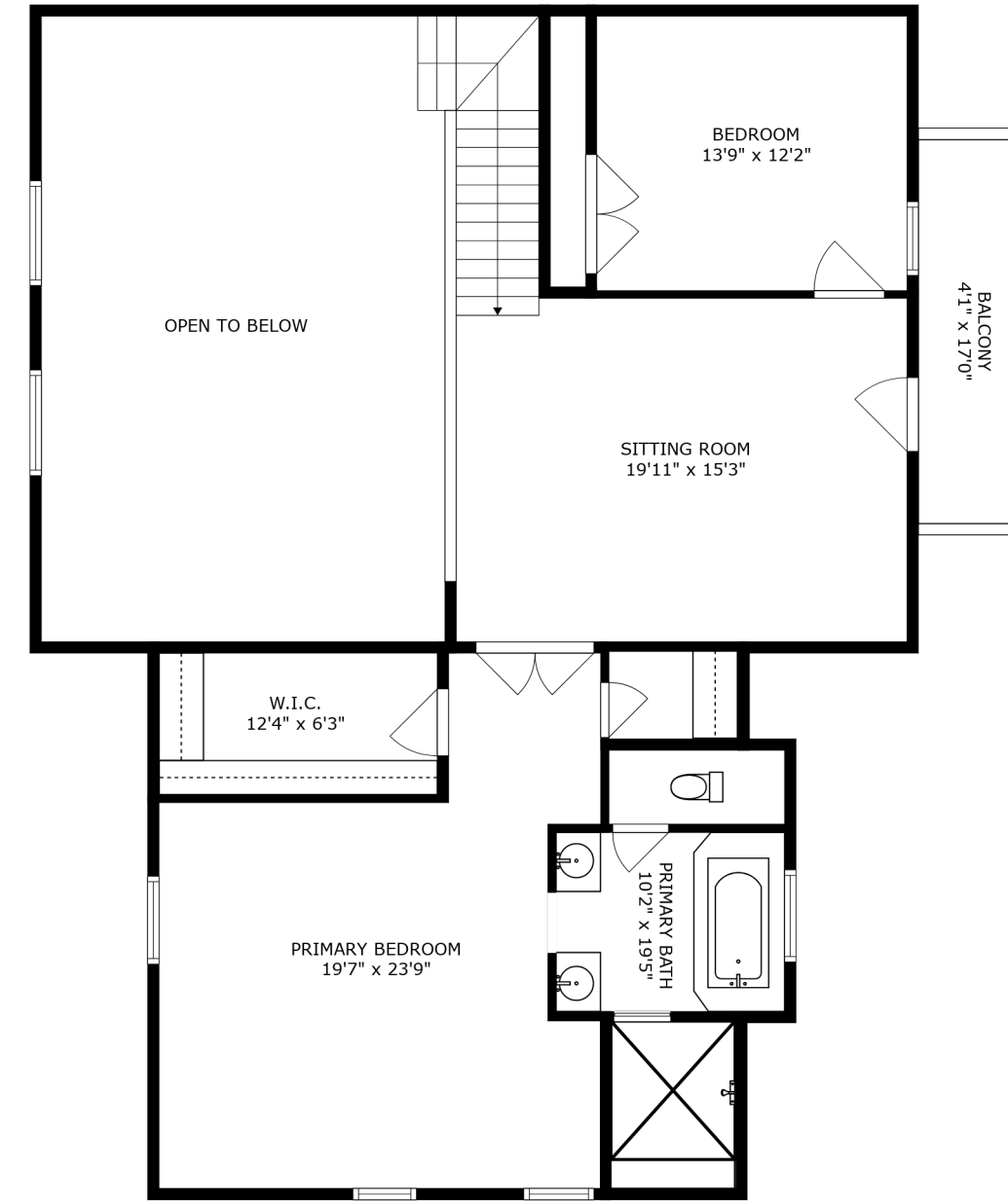
FLOOR 3
