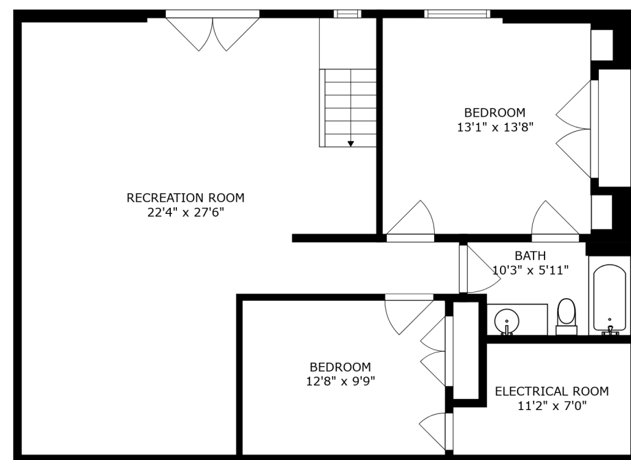
FLOOR 1
