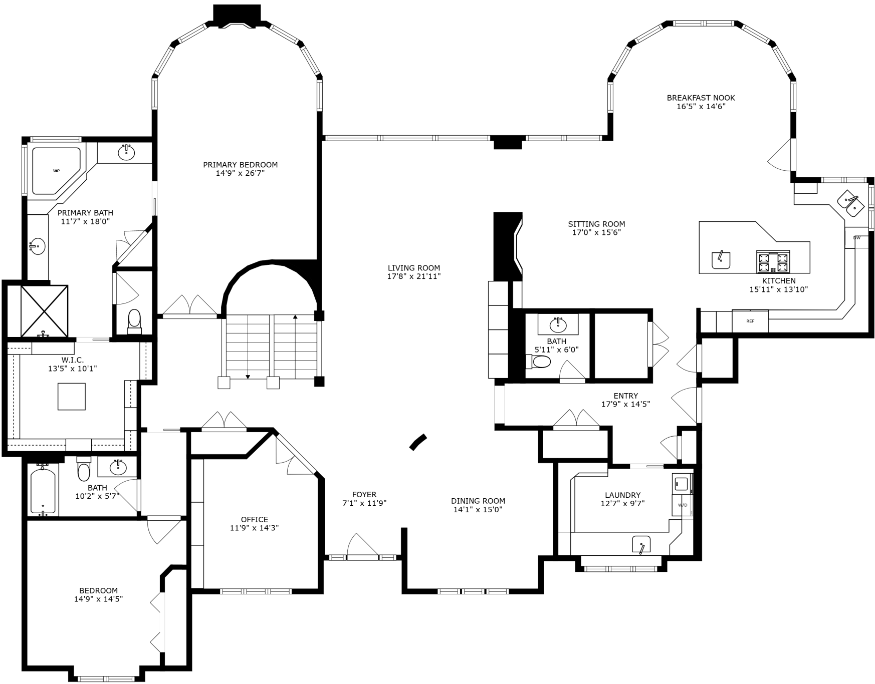
FLOOR 2
