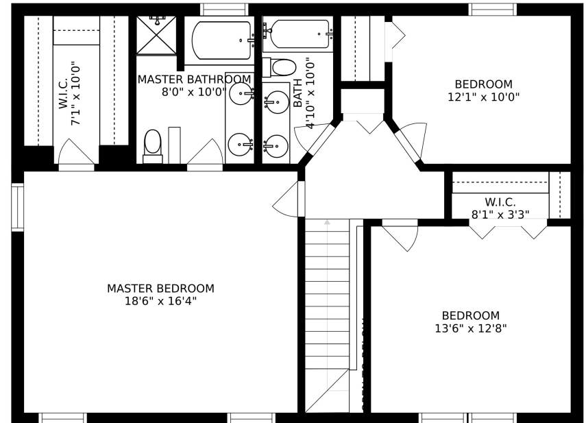
FLOOR 2
