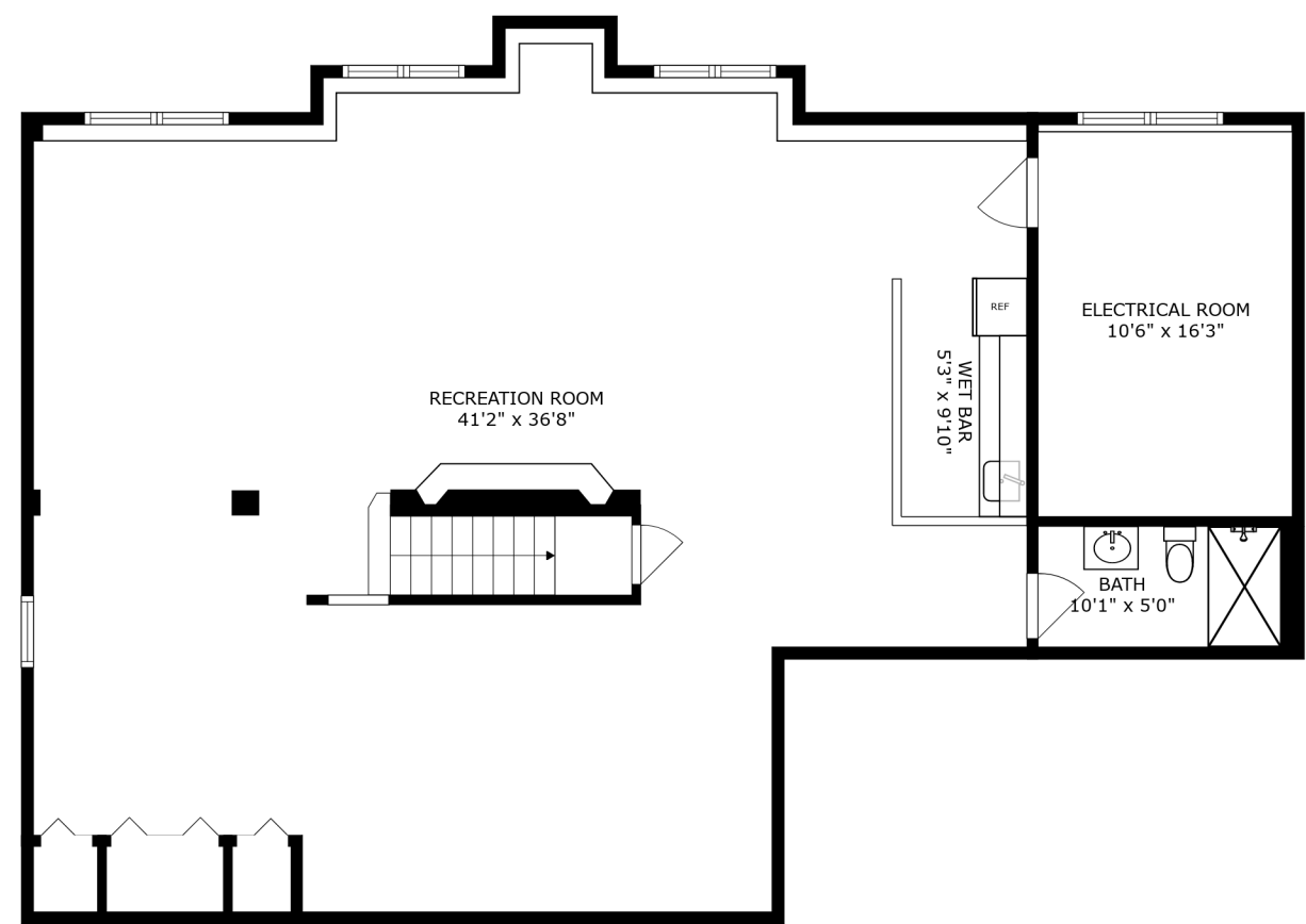
FLOOR 1
