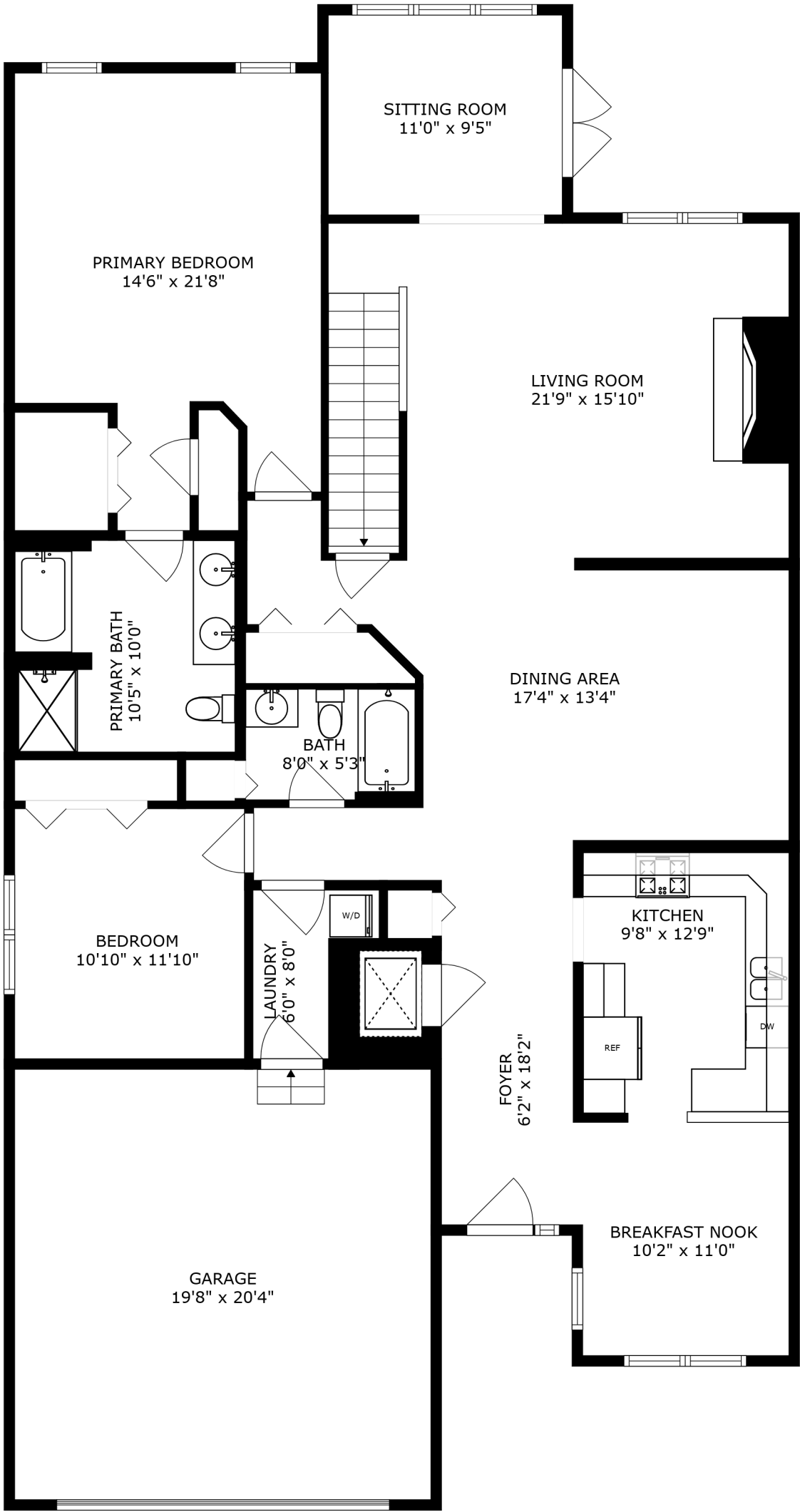
FLOOR 2
