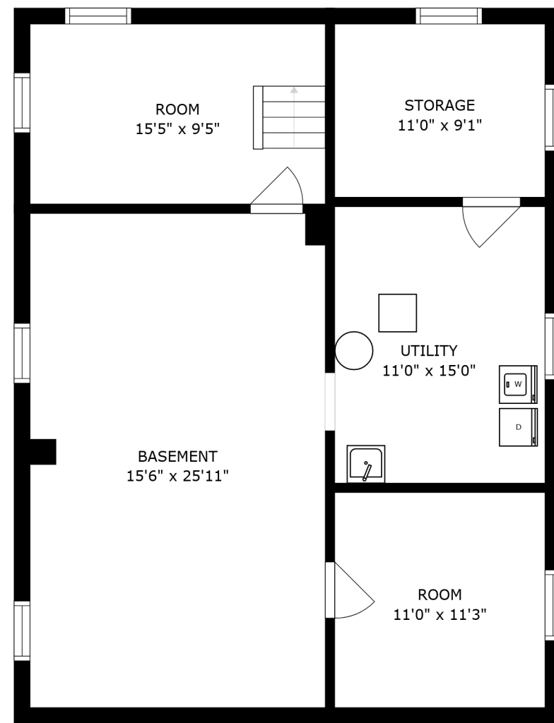
FLOOR 1
