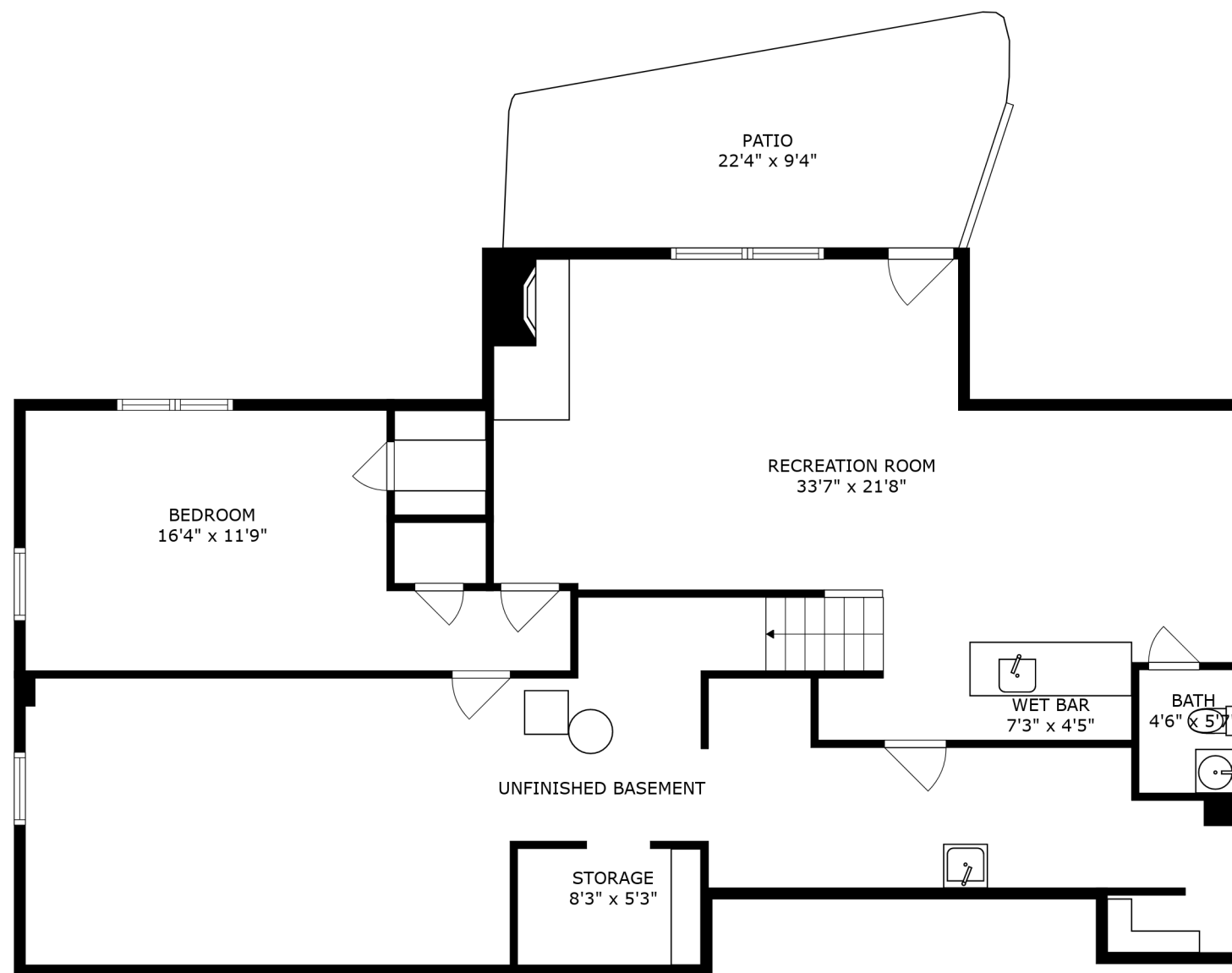
FLOOR 1
