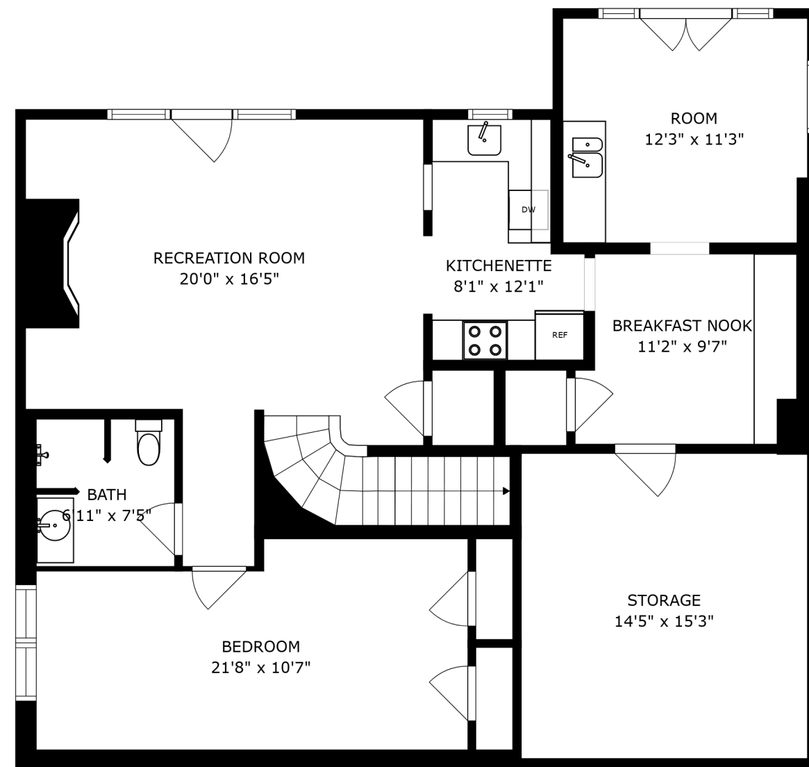
FLOOR 2
