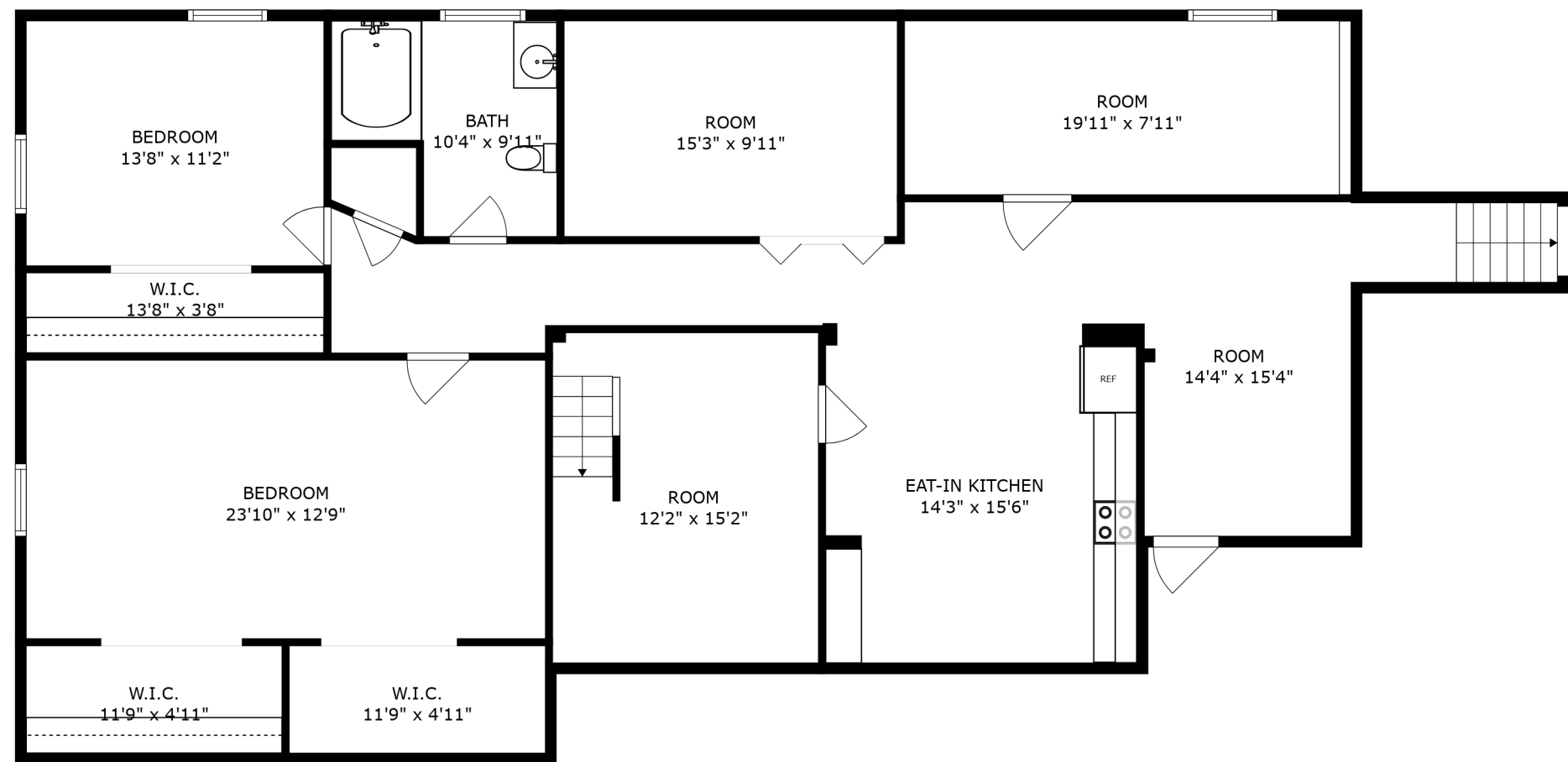
FLOOR 1
