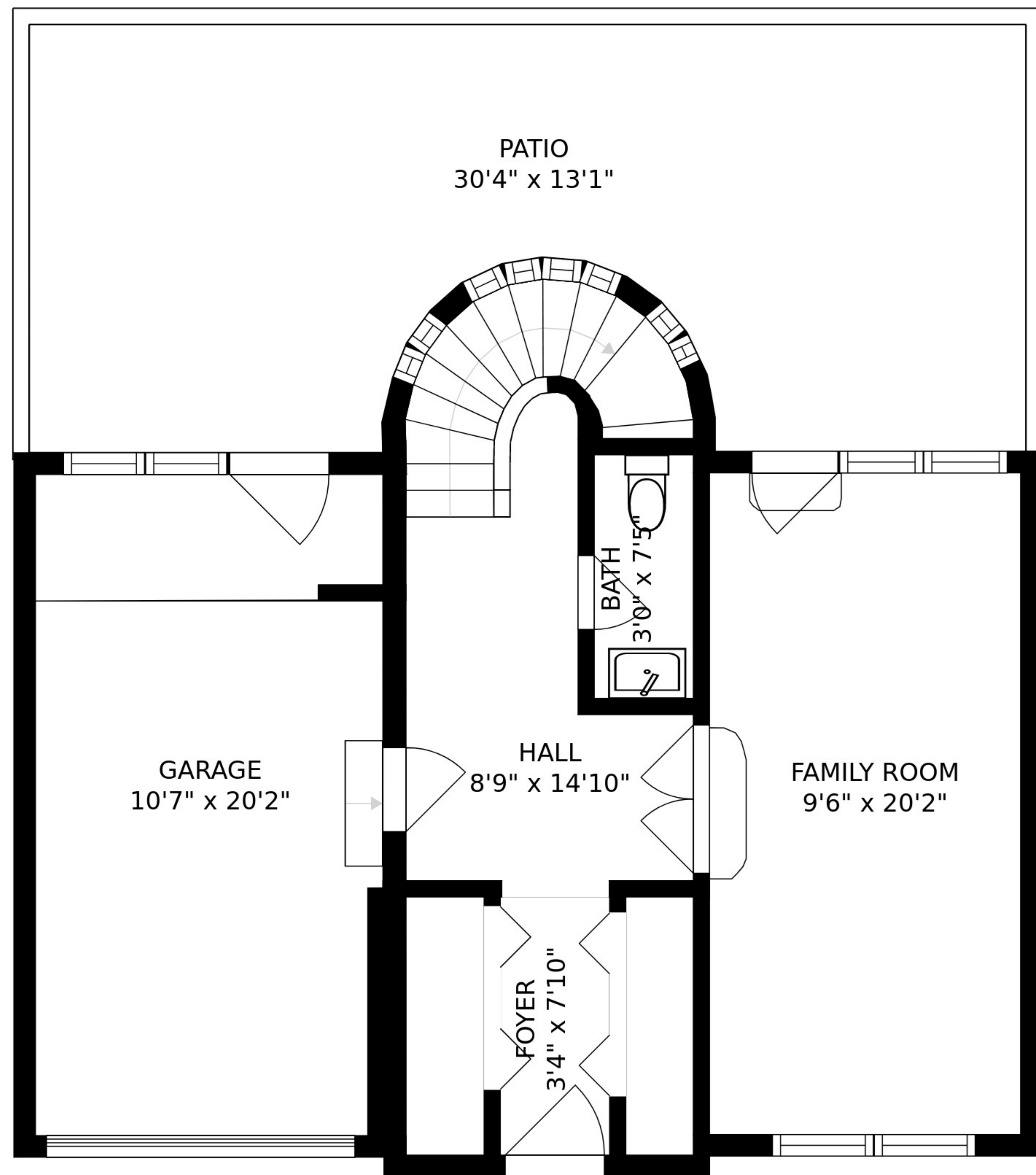
FLOOR 1
