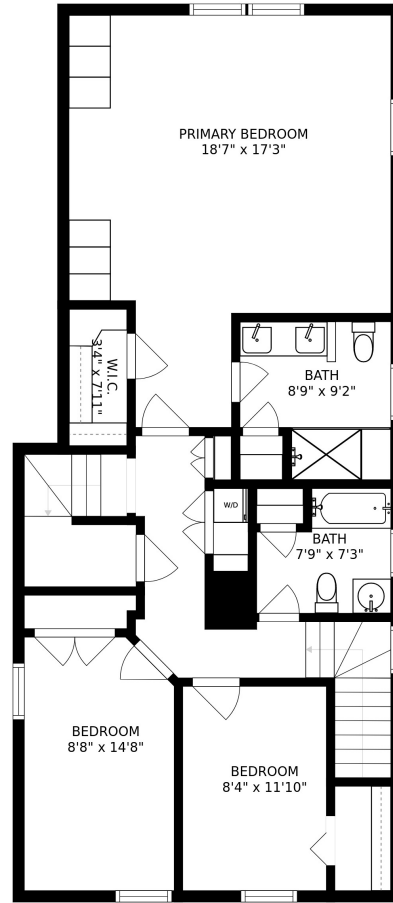
FLOOR 3
