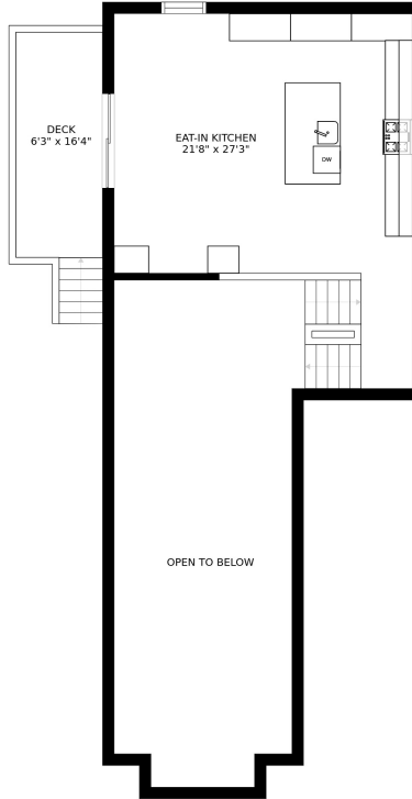
FLOOR 3
