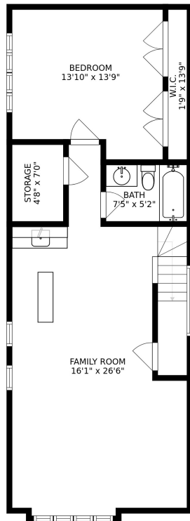
FLOOR 1
