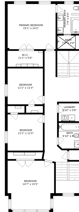
FLOOR 3
