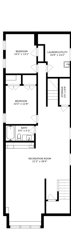
FLOOR 1
