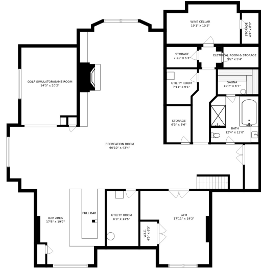
FLOOR 1
