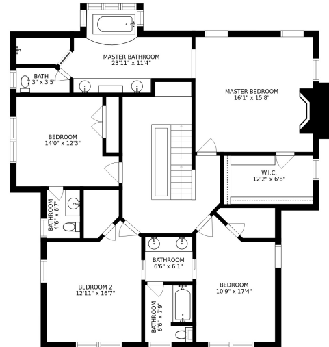
FLOOR 3
