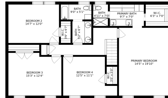
FLOOR 2 CEILING HT. 8'0" APPROX. INTERIOR SQ. FOOTAGE - 1,309
