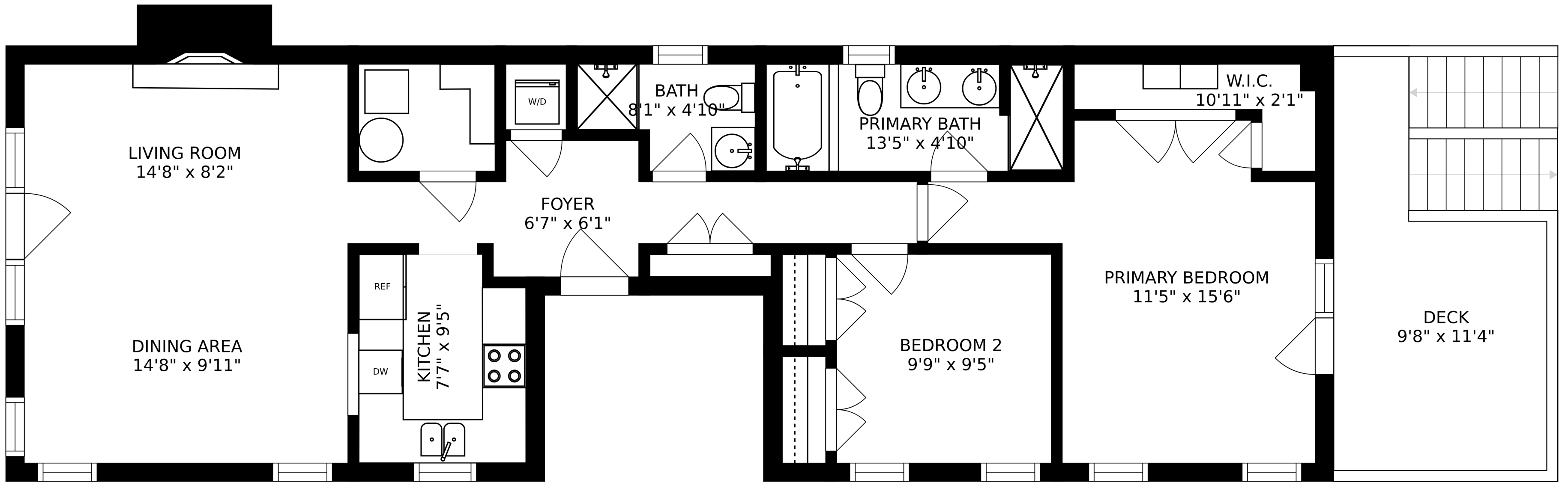
FLOOR 1
